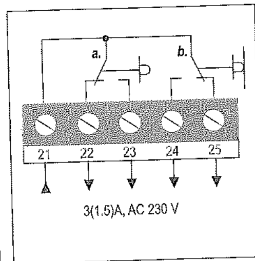
Figure 6: Auxiliary switches
