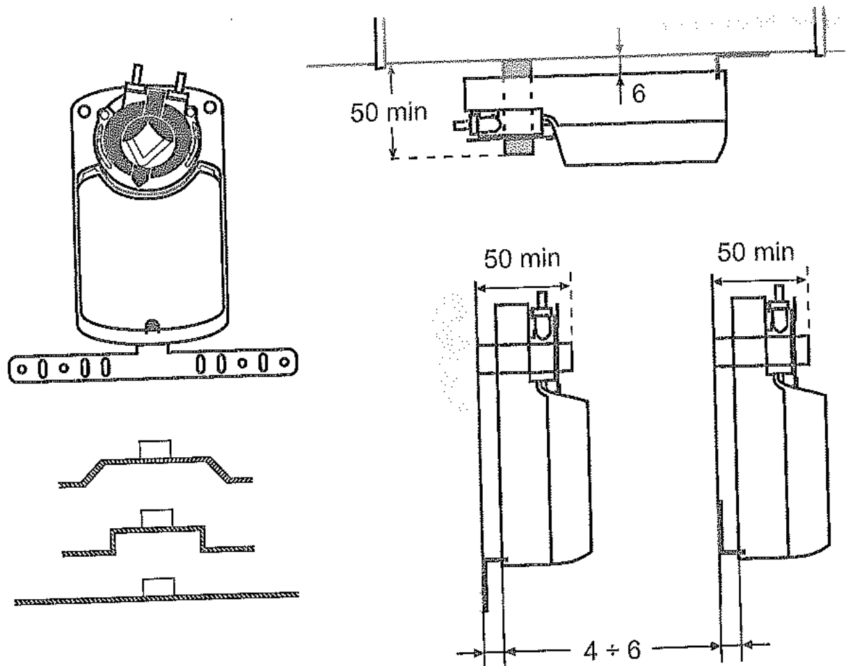
Figure 3: Mounting Instructions
