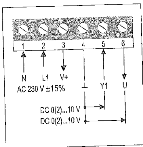
Figure 4: Proportional Control
