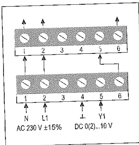
Figure 5: Parallel Connection
